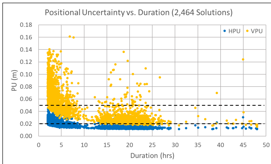
Figure 2: Positional Uncertainty (PU) vs. duration for the entire dataset.
