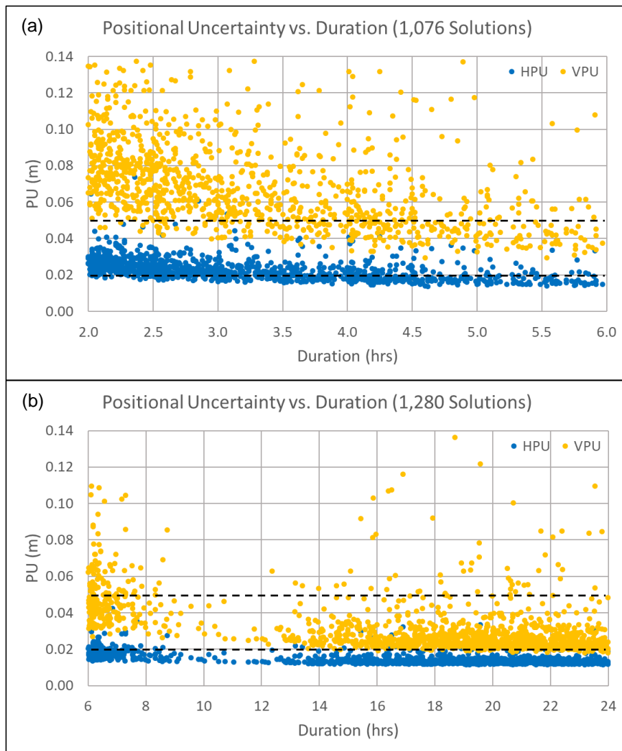
Figure 3: Positional Uncertainty (PU) vs. duration for (a) 2-6 hour data, and (b) 6-24 hour data.
