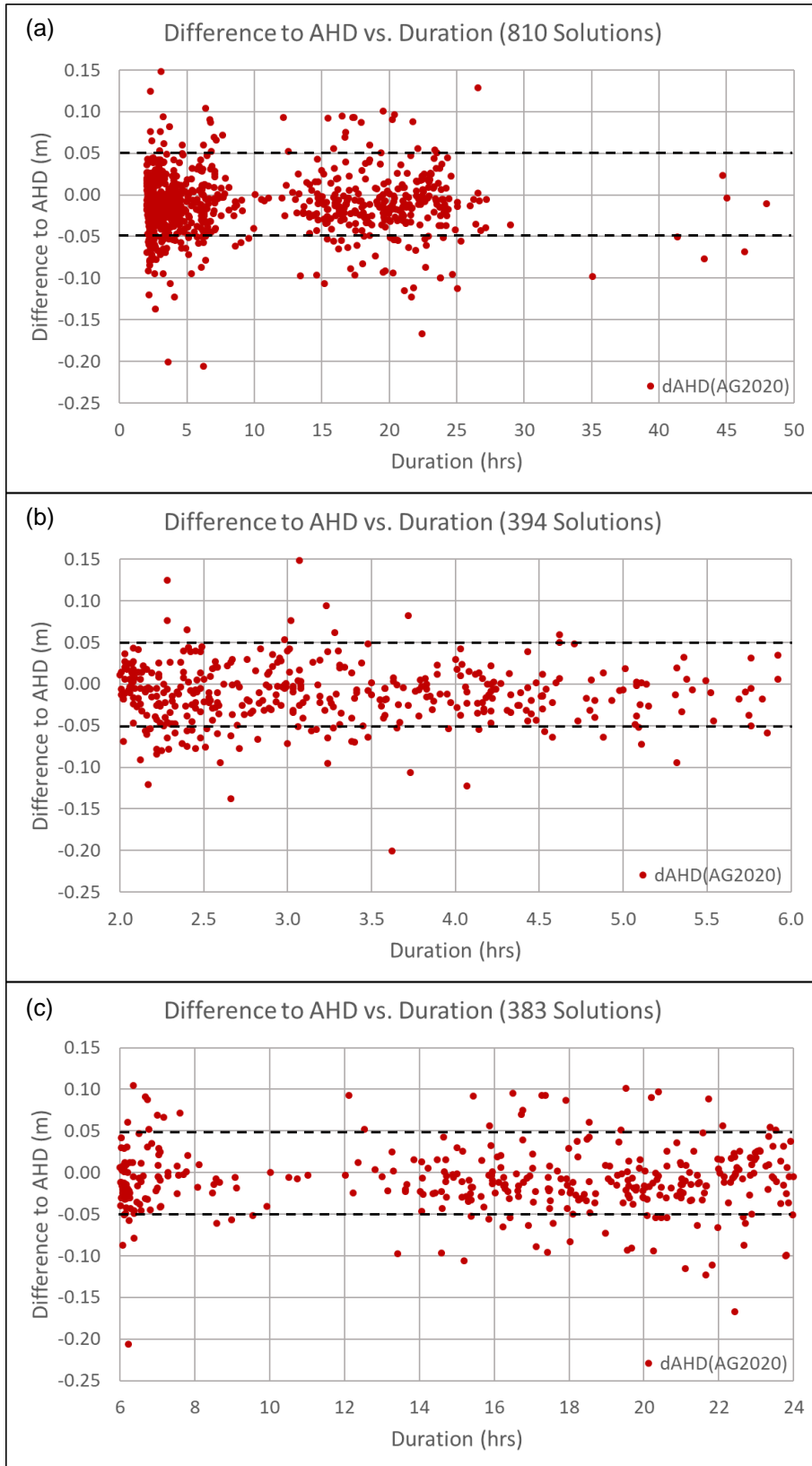
Figure 11: Agreement to levelled AHD vs. duration for (a) the entire subset, (b) 2-6 hour data, and (c) 6-24 hour data.
