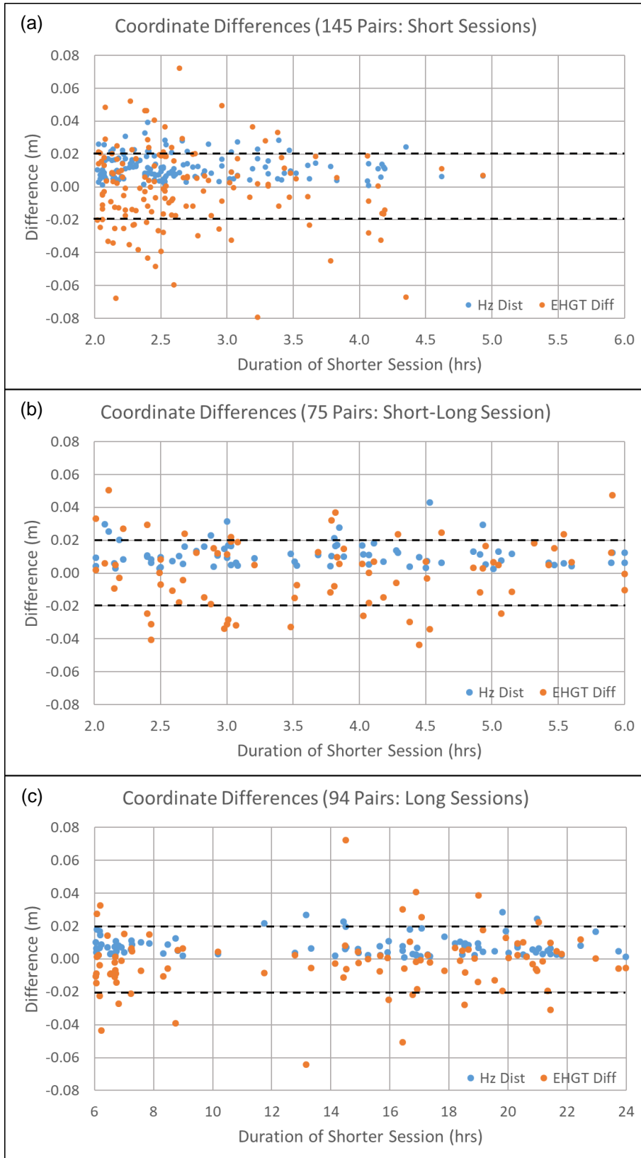
Figure 6: Difference in horizontal and vertical coordinates vs. duration for (a) 145 short-session pairs, (b) 75 short-long-session pairs, and (c) 94 long-session pairs.
