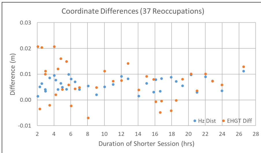
Figure 8: Difference in horizontal and vertical coordinates vs. duration for TS3663 PANORAMA.
