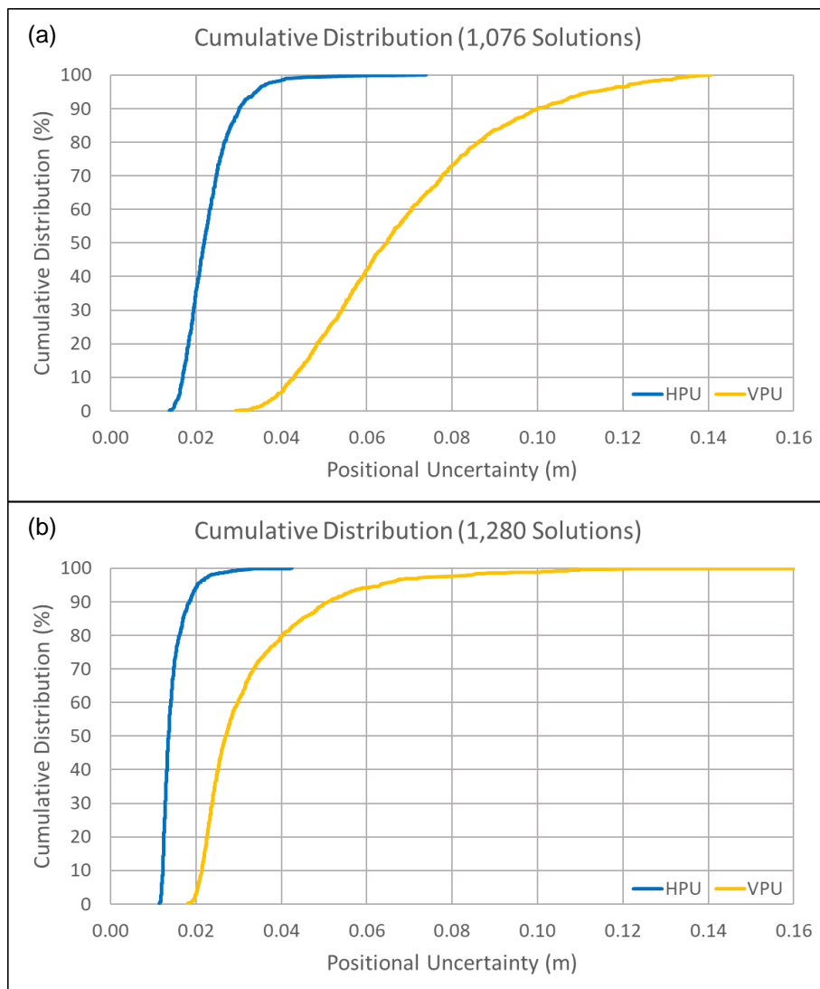
Figure 5: Cumulative distribution of PU for (a) the 2-6 hour data, and (b) 6-24 hour data.
