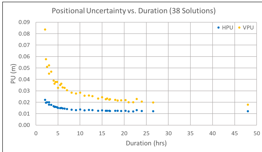
Figure 10: Positional Uncertainty (PU) vs. duration for TS3663 PANORAMA.
