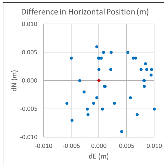
Figure 9: Difference in horizontal position from 48-hour solution for TS3663 PANORAMA (37 reoccupations).
